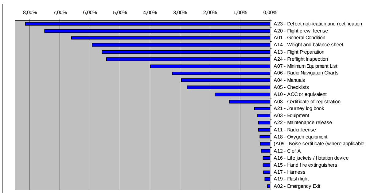
Ratio Number of Findings per Inspections: Flight Deck Items
