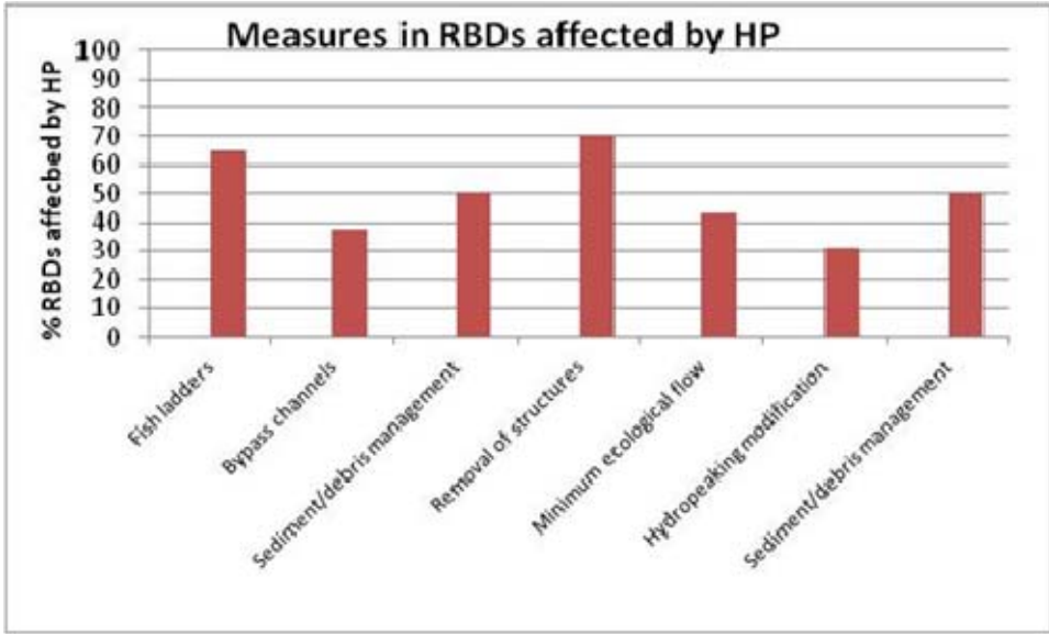
Figure 8.14.5: Measures related to hydropower installations
