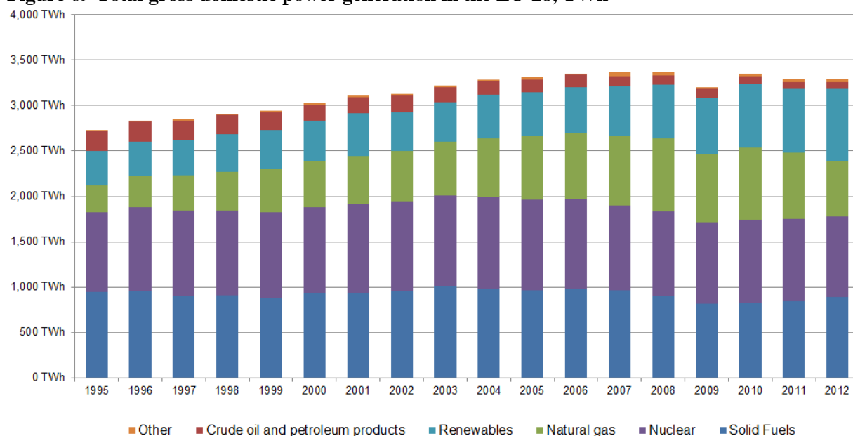
Figure 69 Total gross domestic power generation in the EU-28, TWh
