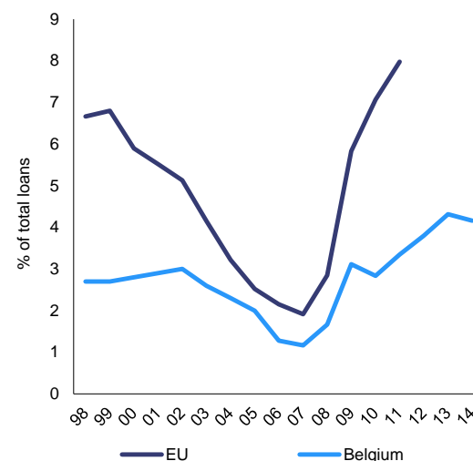
Graph 2.4.6: Non-performing loans
