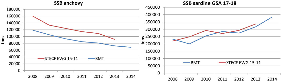
Figure A.8 Comparison between BEMTOOL and stock assessment SSB by fleet segment for anchovy and sardine in GSA 17 and 18.
