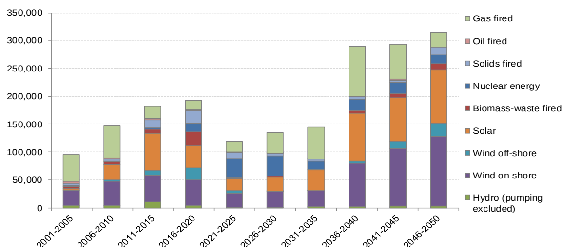
Figure 8: Net power capacity investments by plant type (MWh – for five year period)
