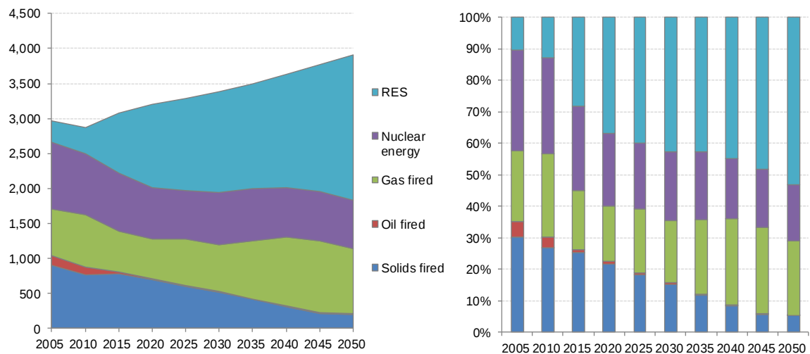
Figure 5: EU power generation (net) by fuel (Mtoe – left, shares – right)
