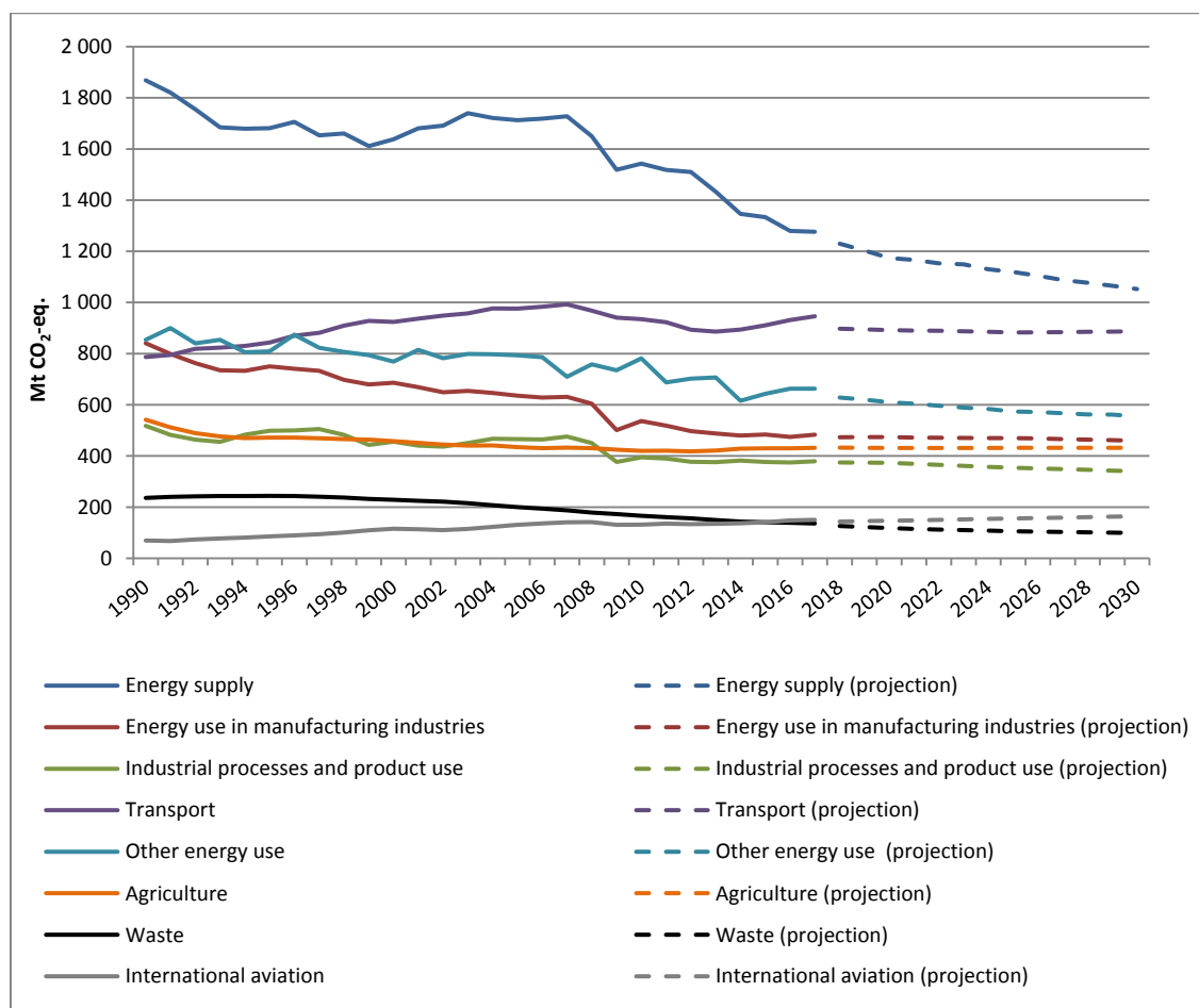
Figure 1: EU greenhouse gas emissions by sector, historical data (1990-2017) and projections (2017-2030). 7
