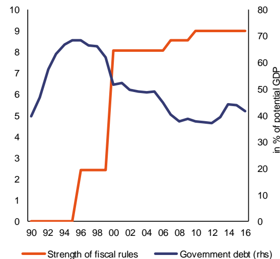
Graph 4.1.3: Swedish fiscal rules index and government gross debt
