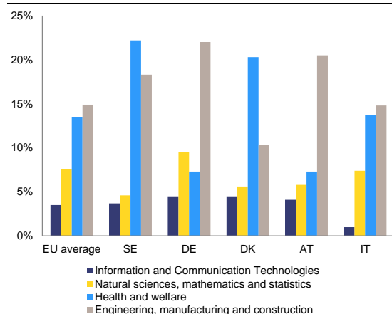
Graph 4.3.6: Proportion of graduates by programme orientation (2016)
