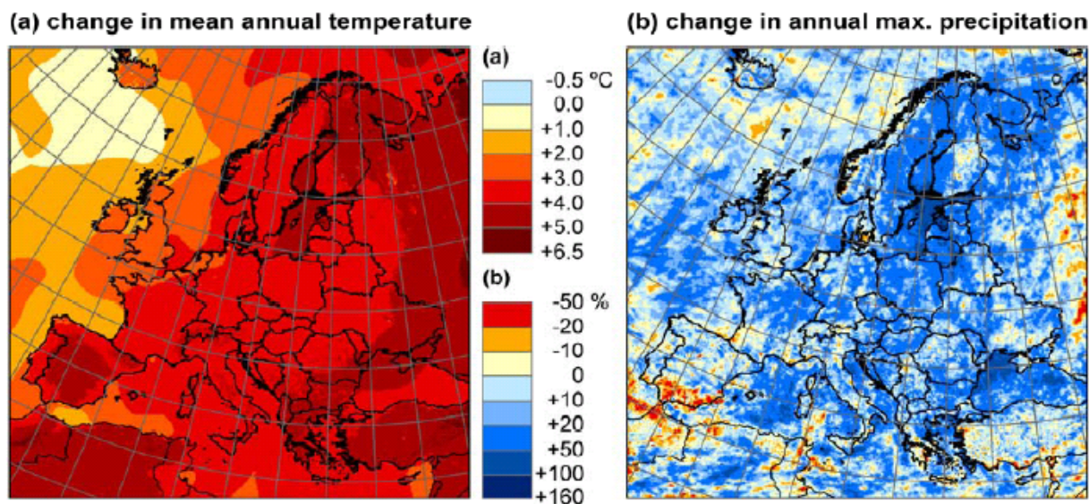
Figure 6: Absolute change in mean temperature (a) and relative change (scenario divided by control) in annual maximum precipitation (b) over Europe as simulated by the regional climate model HIRHAM (scenario A2, resolution 12 km).
