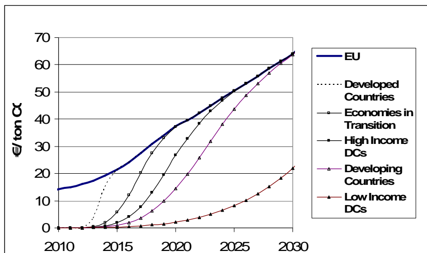
Figure 14: Carbon price differentials between different regions and over time
