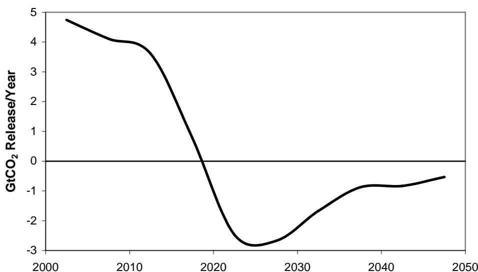
Figure 25: Climate change mitigation scenario in the Land Use Change sector induced by a carbon price
