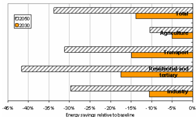
Figure 18: Energy saving per sector relative to baseline (JRC-IPTS, POLES model)
