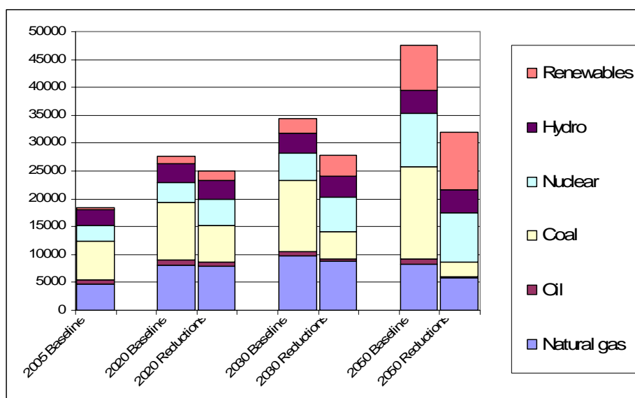
Figure 22: Development of the importance of different fuel types in the electricity generation mix (in TWh), POLES model results
