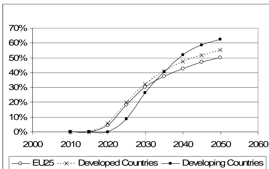
Figure 21: Share of Power Sector Emissions Captured (JRC-IPTS, POLES)
