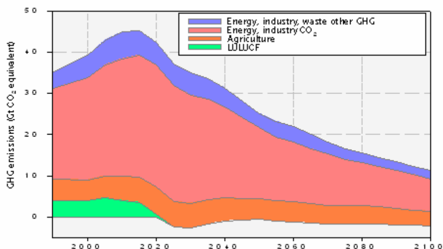
Figure 11: Global greenhouse gas emissions to meet 2 degrees C with 50% probability, (JRC/IPTS)
