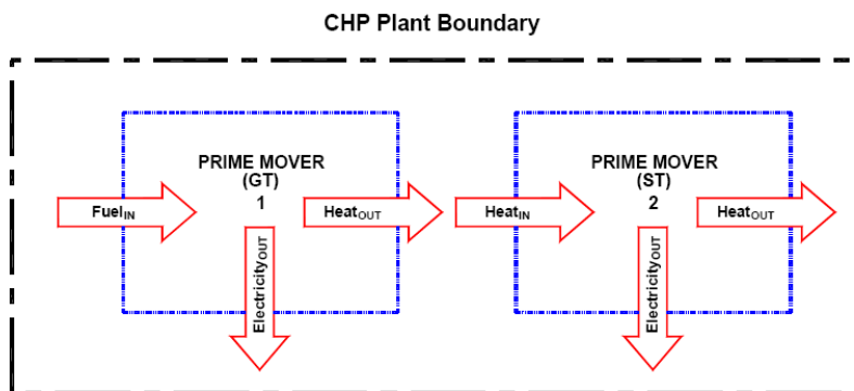
Figure 5: Boundary of cogeneration unit for connected prime movers.
