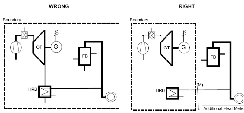
Figure 3: Selection of the correct system boundaries in case of auxiliary/stand by boilers (GT: Gas Turbine; G: Generator; FB: Fuel Boiler; HRB: Heat Recovery Boiler)
