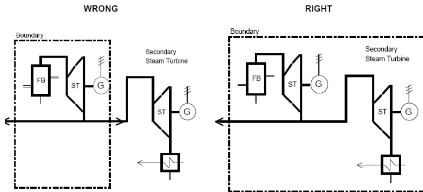
Figure 4: Selection of the correct system boundaries in the case of secondary steam turbines (ST: Steam Turbine)
