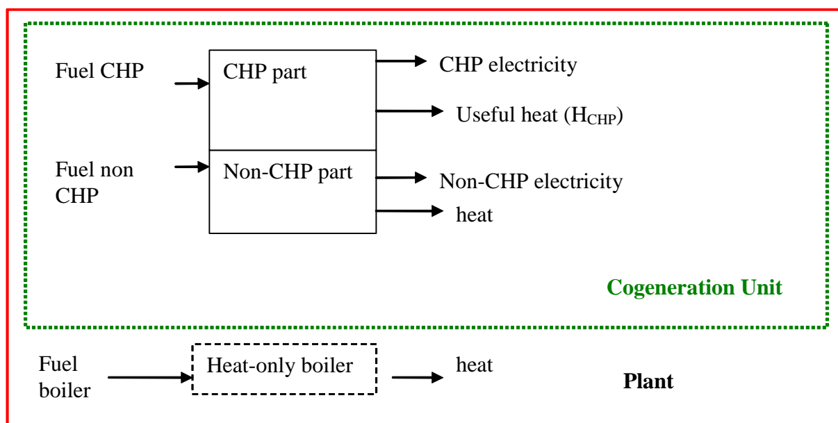
Figure 1: CHP part, non-CHP part and heat-only boilers within a plant
